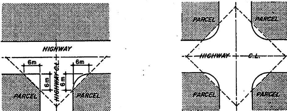
Sight Triangle (not to scale)
